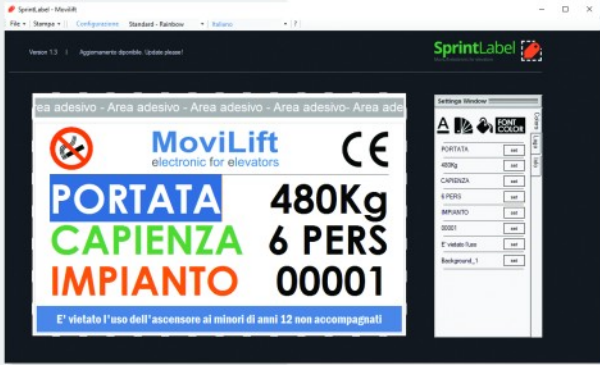
Software Sprintlabel
