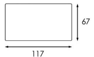
Flush mounting cut-out
