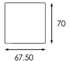
Frame mounting cut-out
