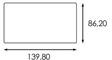
Frame mounting cut-out
